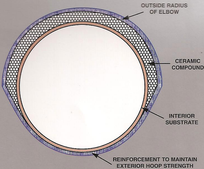
Cross Section of Elbow
